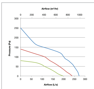
Performance - MF100
