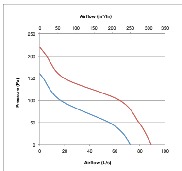
Performance - MF125
