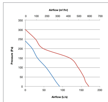
Performance - MF150
