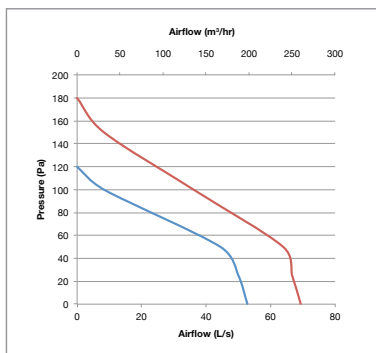
Performance - MF100
