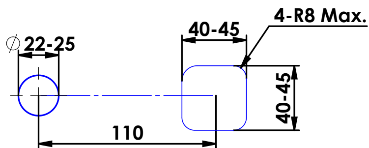
Mounting Hole
