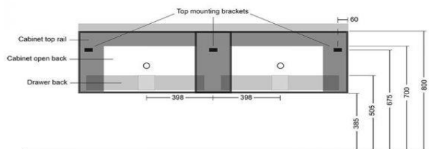
Rear View (KZCS1600_) 1600mm wide x 470mm deep x 415mm high
