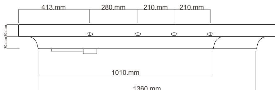
BACK WASHBASIN VIEW
