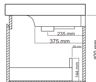
SIDE WASHBASIN VIEW
