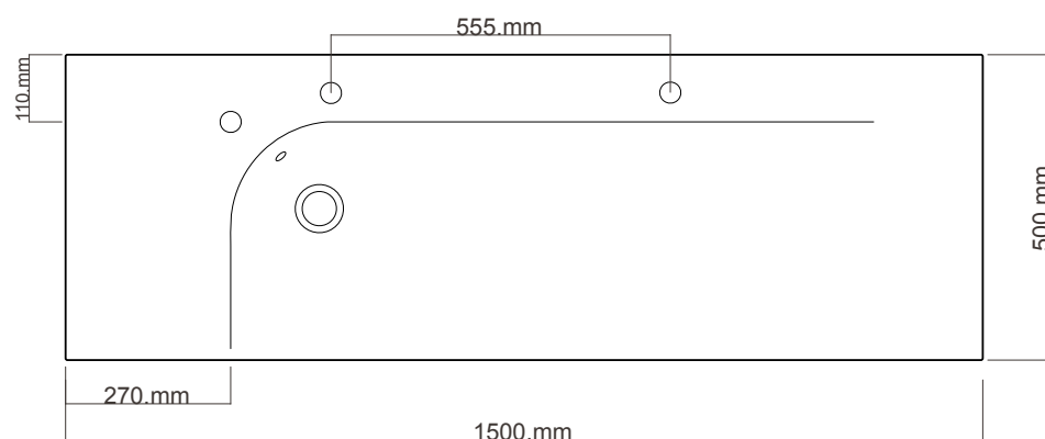
TOP WASHBASIN VIEW
