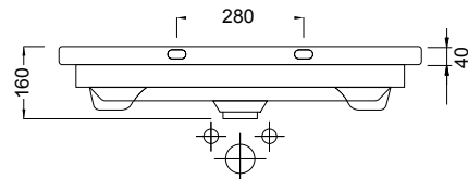
Back Section Basin
