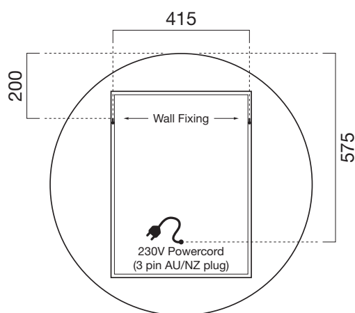
Mounting Dimensions
