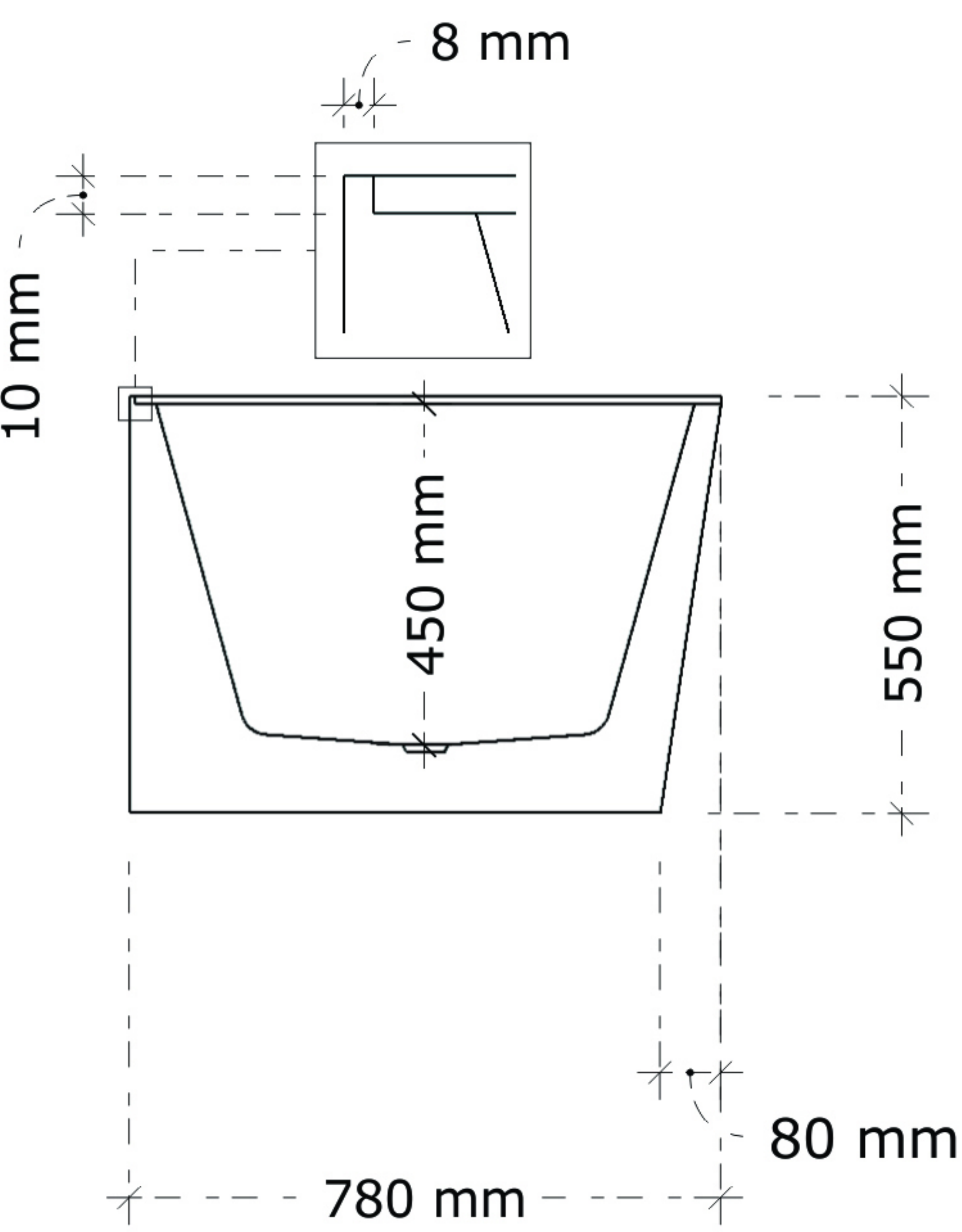
LEFT SIDE VIEW
