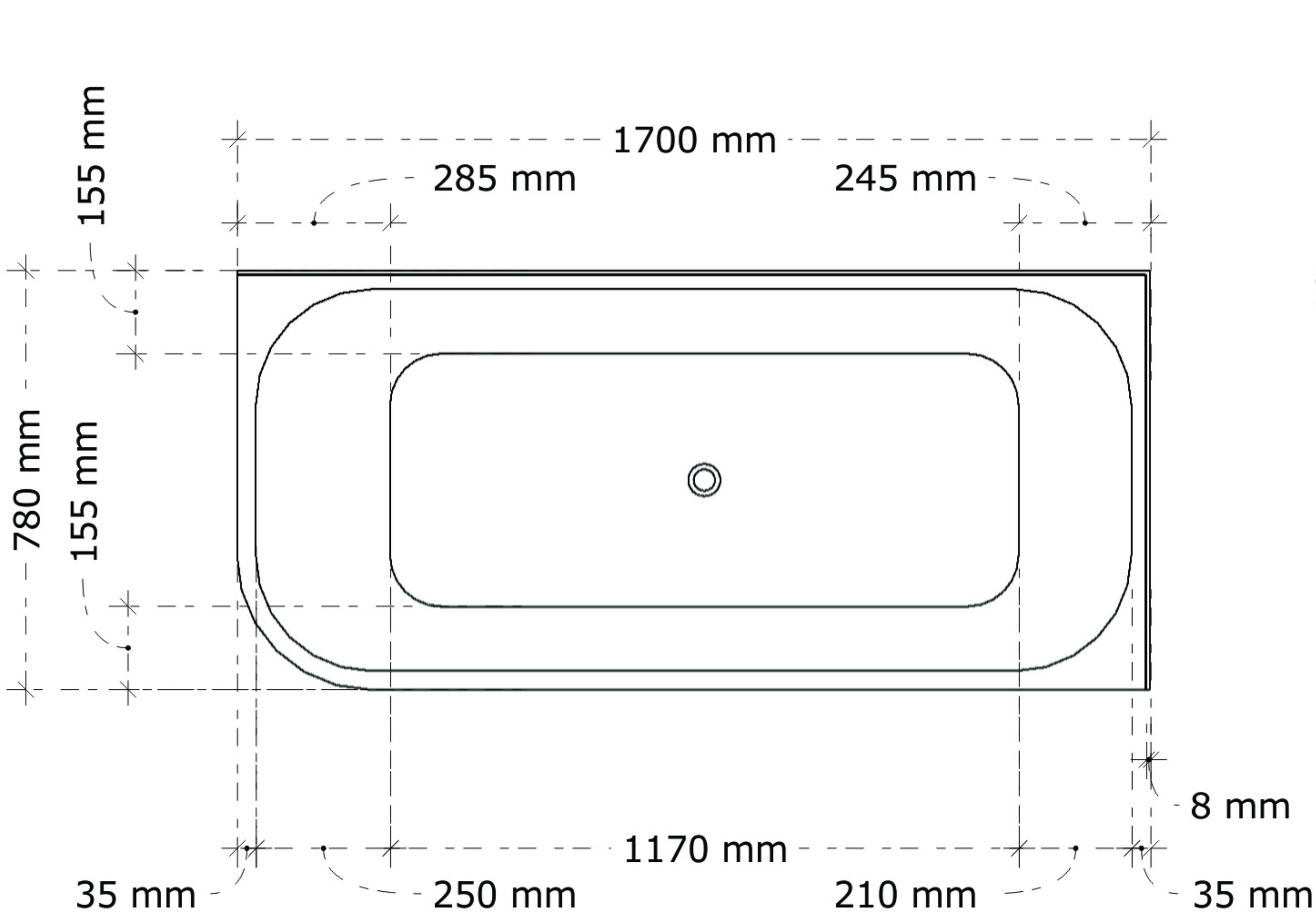
TOP VIEW
