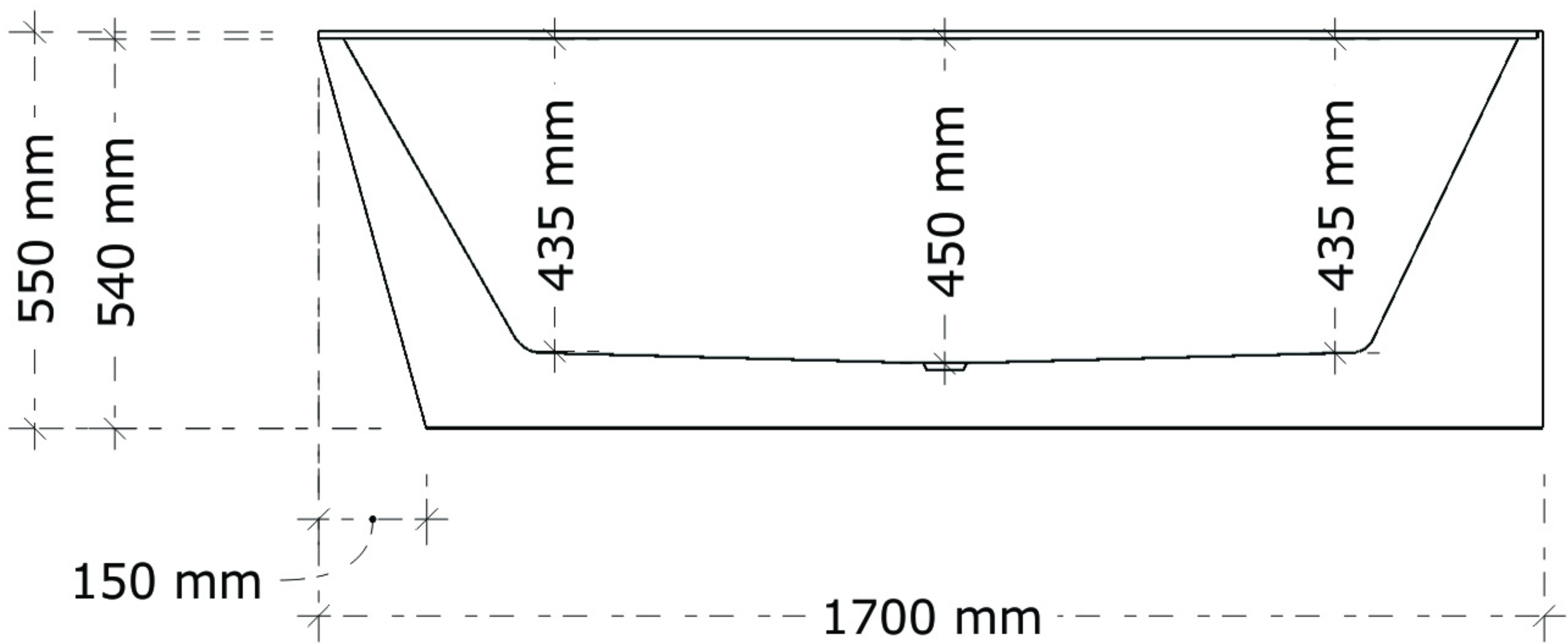
FRONT VIEW
