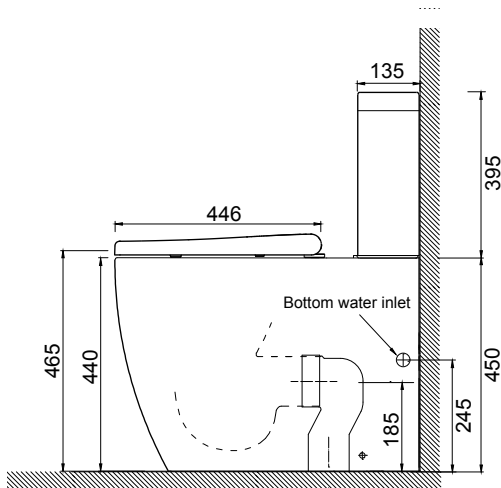
RH Side Section
