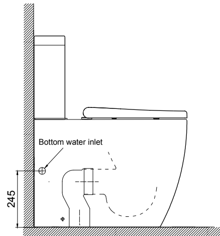
LH Side Section
