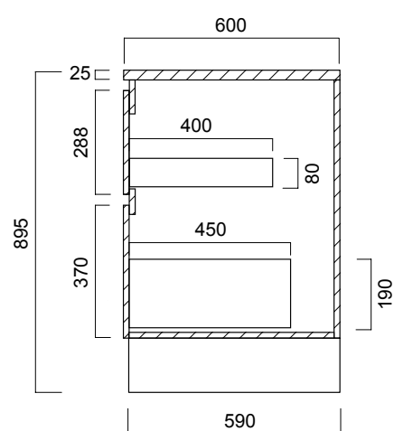
Side Section (Melamine)
