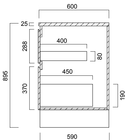
Side Section (Painted & Timber Veneer)
