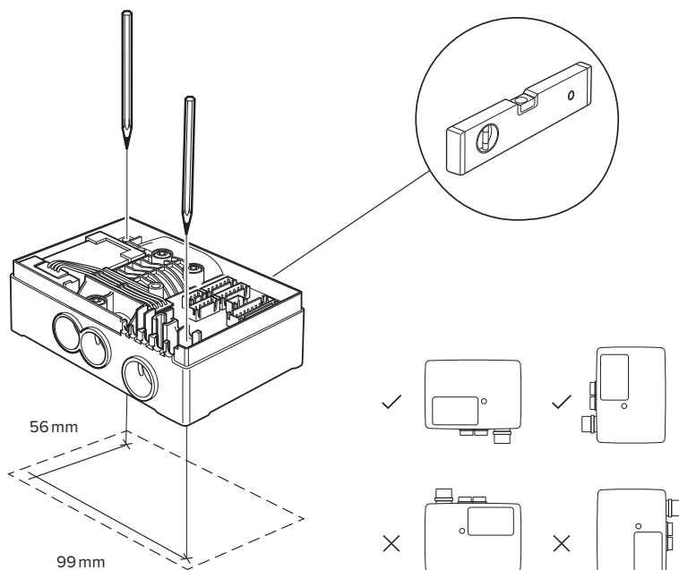
1 Mark fixing holes
