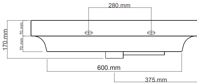
BACK WASHBASIN VIEW
