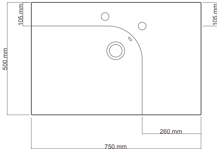
TOP WASHBASIN VIEW
