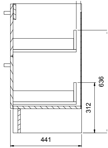
SPLASH Floor Drawer Units Side View
