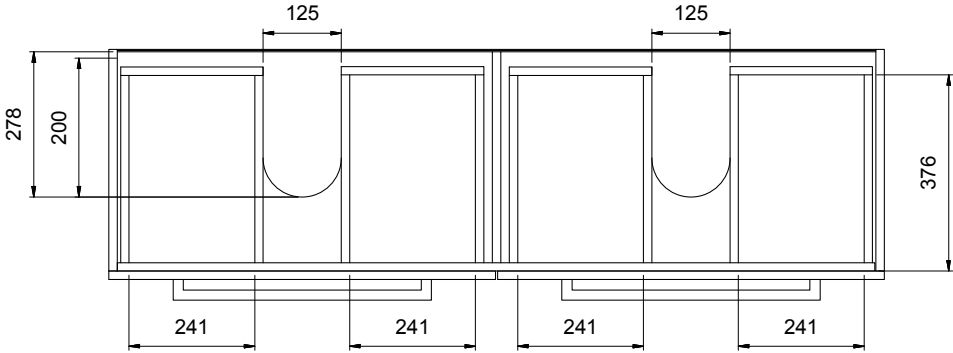
SP150D4FLDB Top View Showing Drawers
