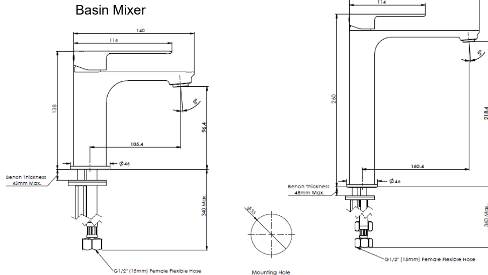
Tower Basin Mixer
