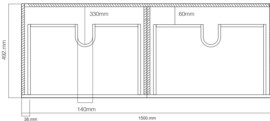
DRAWER
