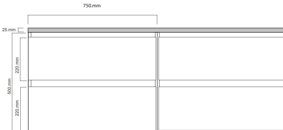
FRONT VIEW
